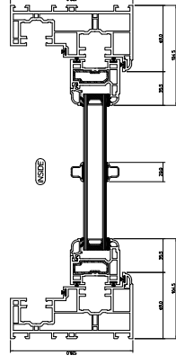
Downwards View - Bottom Sash
