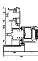
Sideways View - Standard Bottom Rail
