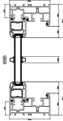
Downwards View - Top Sash
